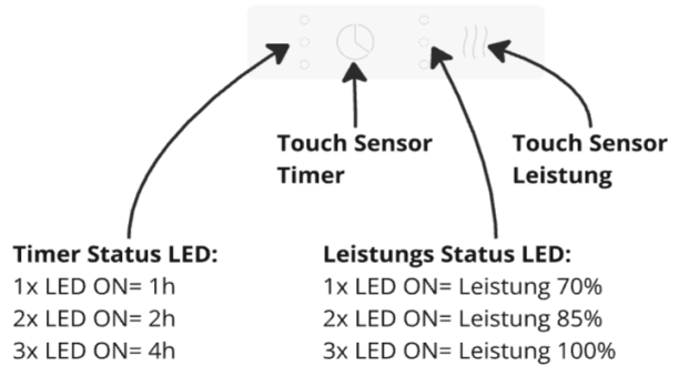
Abb. 12: Touch sensor
